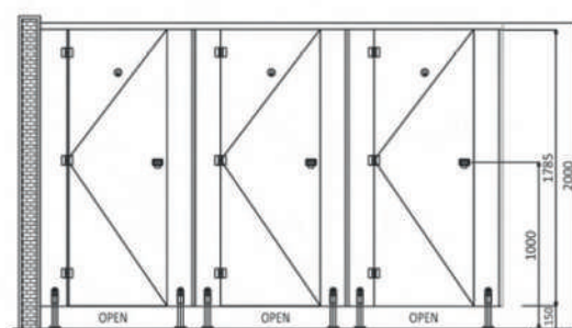
Front View (CU)
