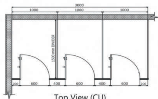
Top View (CU)
