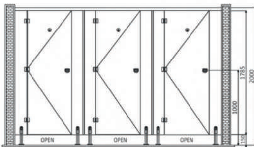
Front View (EU)
