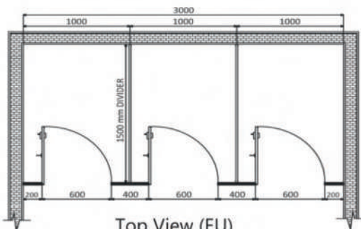
Top View (EU)
